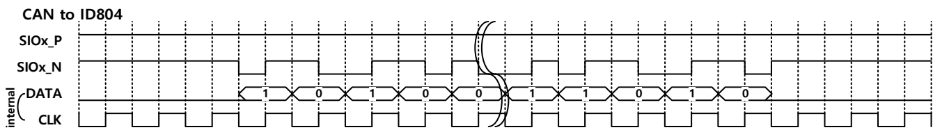
Fig 16. Example of CAN Transceiver to ID804 communication
