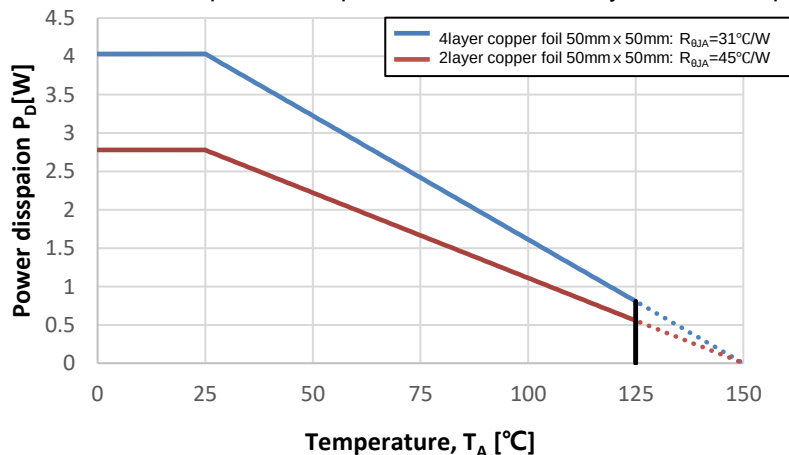
Fig 7. Thermal Considerations
