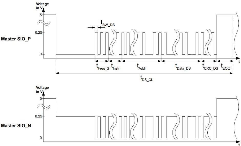
Fig 33. Differential downstream command frame
