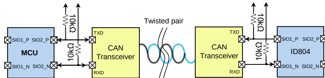
Fig 15. Bi-directional chain example with direct MCU-CAN-FD connection. The MCU needs to implement the Manchester decoder.
