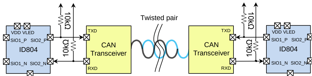
Fig 14. Bi-directional chain example with CAN-FD section. The ID804 serves as Manchester decoder between the chain and the MCU(upstream direction).
